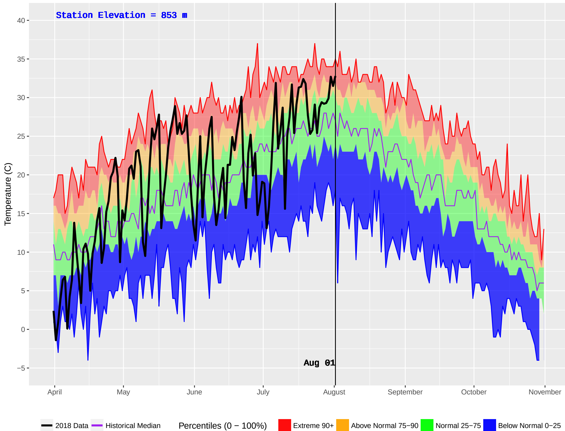
JOHNSON LAKE (419) : Historical (1986–2016) and Current (2018) Daily Temperature
